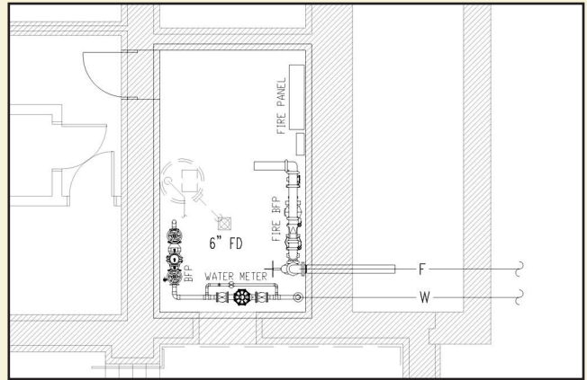
Proposed layout of incoming water service for domestic and fire suppression at the northwest corner of the basement level. As the design continues, this layout will be modified to accommodate all of the requirements of a fully modernized building.
